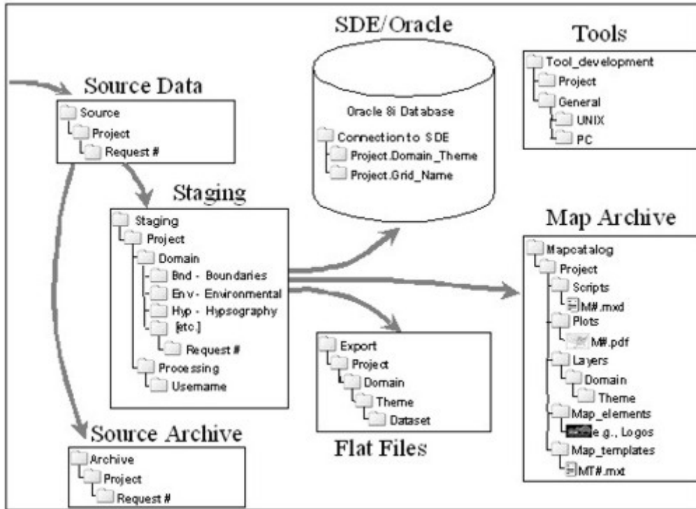
Figure 4. The logical data architecture of the CGRP-GIS.
