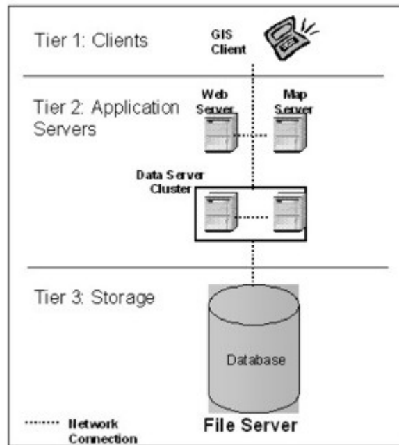
Figure 5. The three-tier architecture of the CGRP-GIS.
