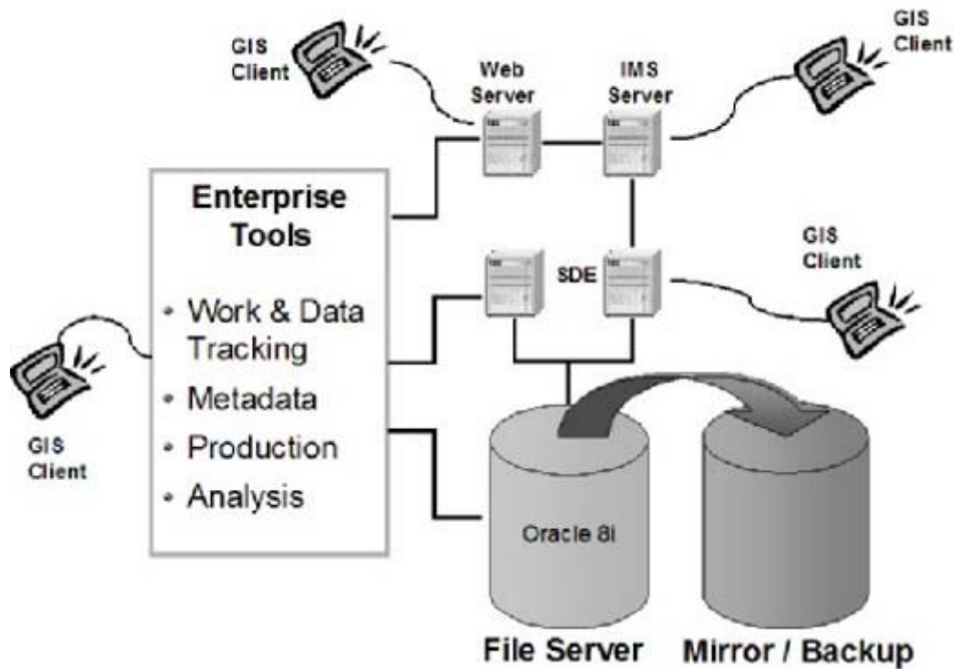
Figure 3. The CGRP-GIS spatial data warehouse physical architecture.
