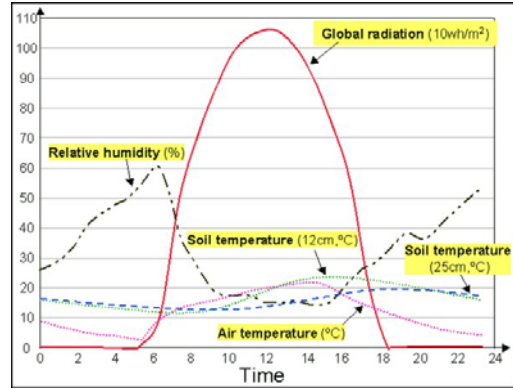
Average diurnal microclimate records for Rocky Mountain Biological Laboratory.
