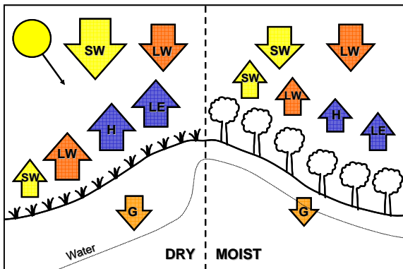
Energy Balance Components: shortwave radiation (SW), longwave radiation (LW), sensible heat (H), latent energy (LE), and storage (G).
