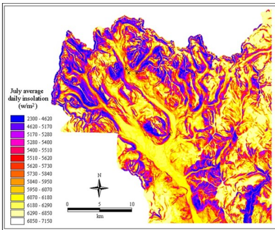
Insolation models for the vicinity of Rocky Mountain Biological Laboratory.
