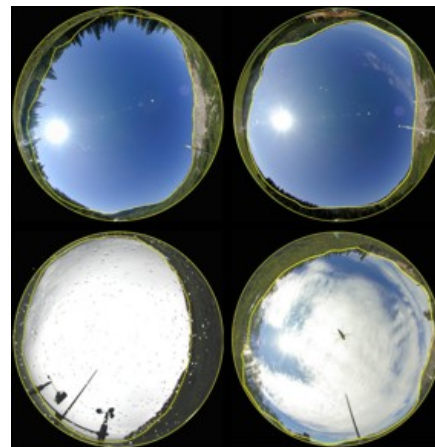
Upward-looking hemispherical photographs of topographic influences on insolation.
